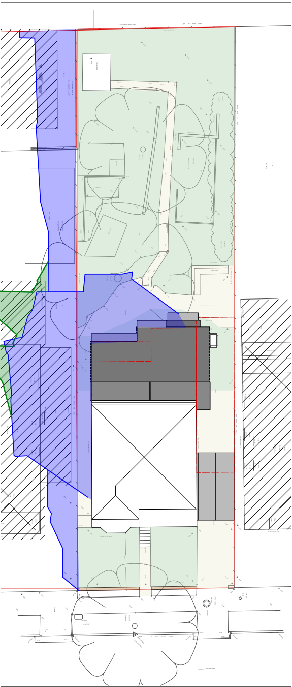
1 3PM WINTER SOLSTICE SOLAR ANALYSIS PLAN Scale: 1:200
